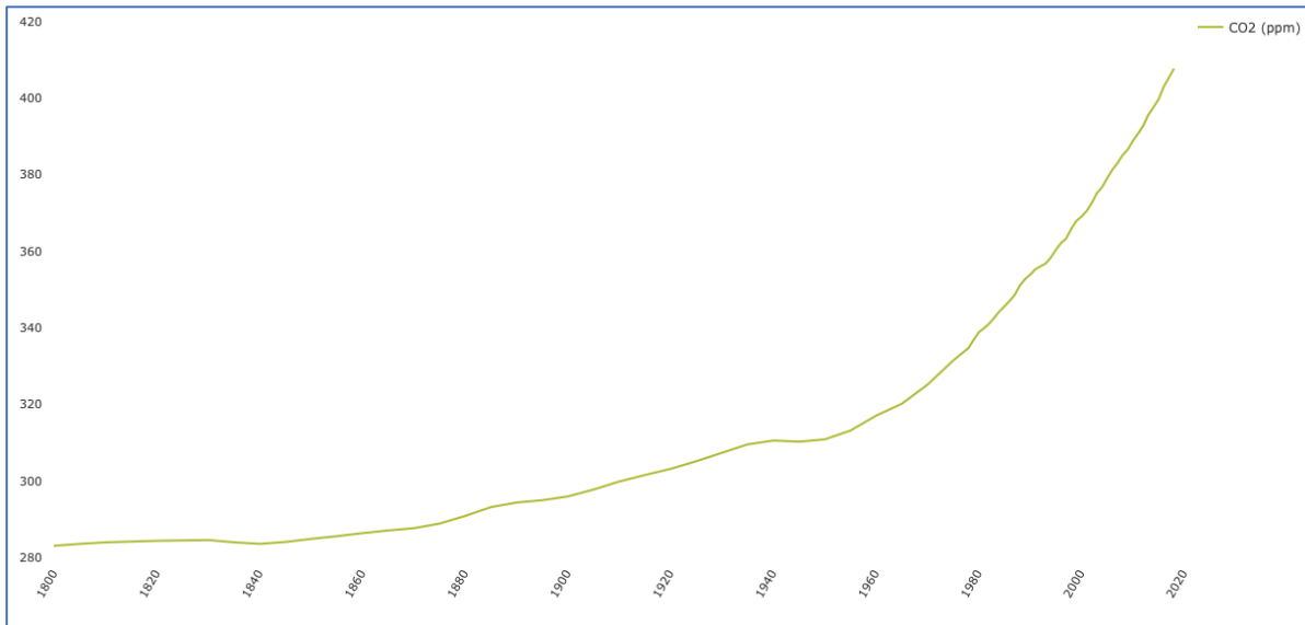
Figure 3. Concentration of CO 2 in the atmosphere
